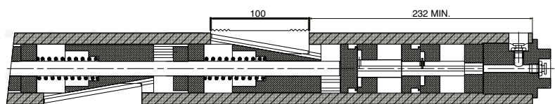
PNEUMO - MECCANICO 3" | PNEUMO - MECHANICAL SHAFT 3"
