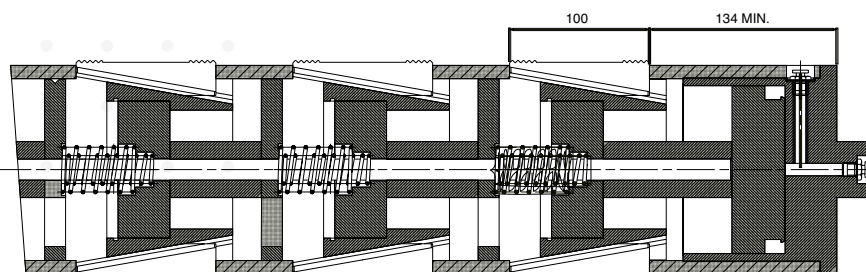
PNEUMO - MECCANICO 6" | PNEUMO - MECHANICAL SHAFT 6"
