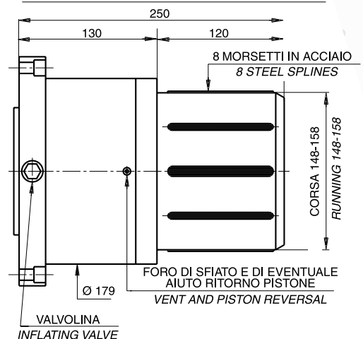
AIR EXPANDING MECHANICAL SPRING RETURN HEADER CORE Ø 152
